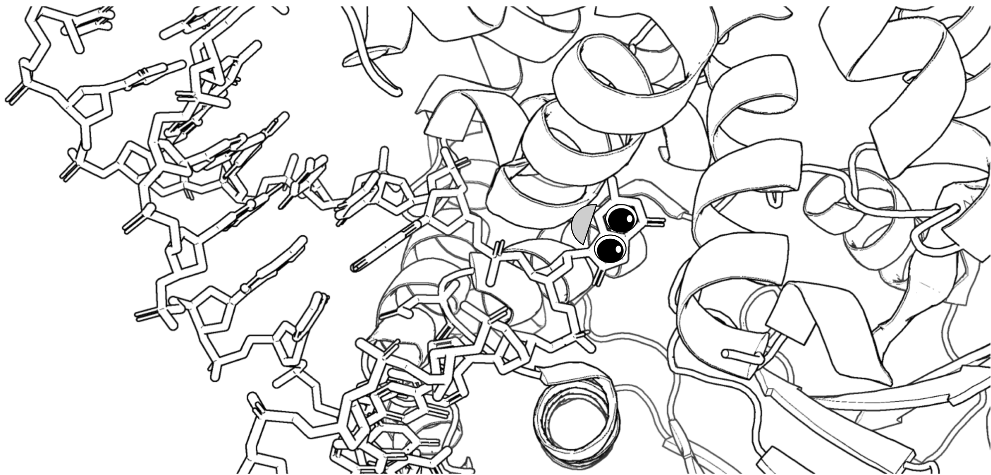
1N3C: hOGG1 thinks oxidized guanines are TERRIFYING(LY CUTE)
